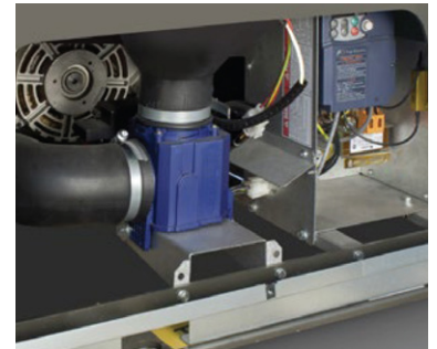
COMPONENT ACCESSIBILITY - FRONT VIEW
